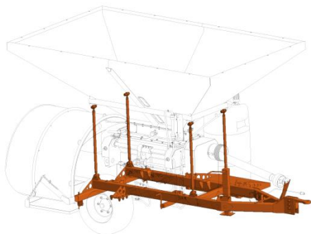
01 FRAME
