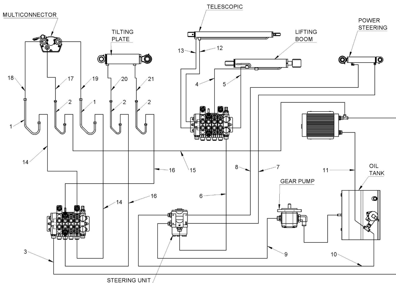
Component list [ TAV. 19 M1 4.2-5.2 HYDRAULIC SERVICES DIAGRAM ]
