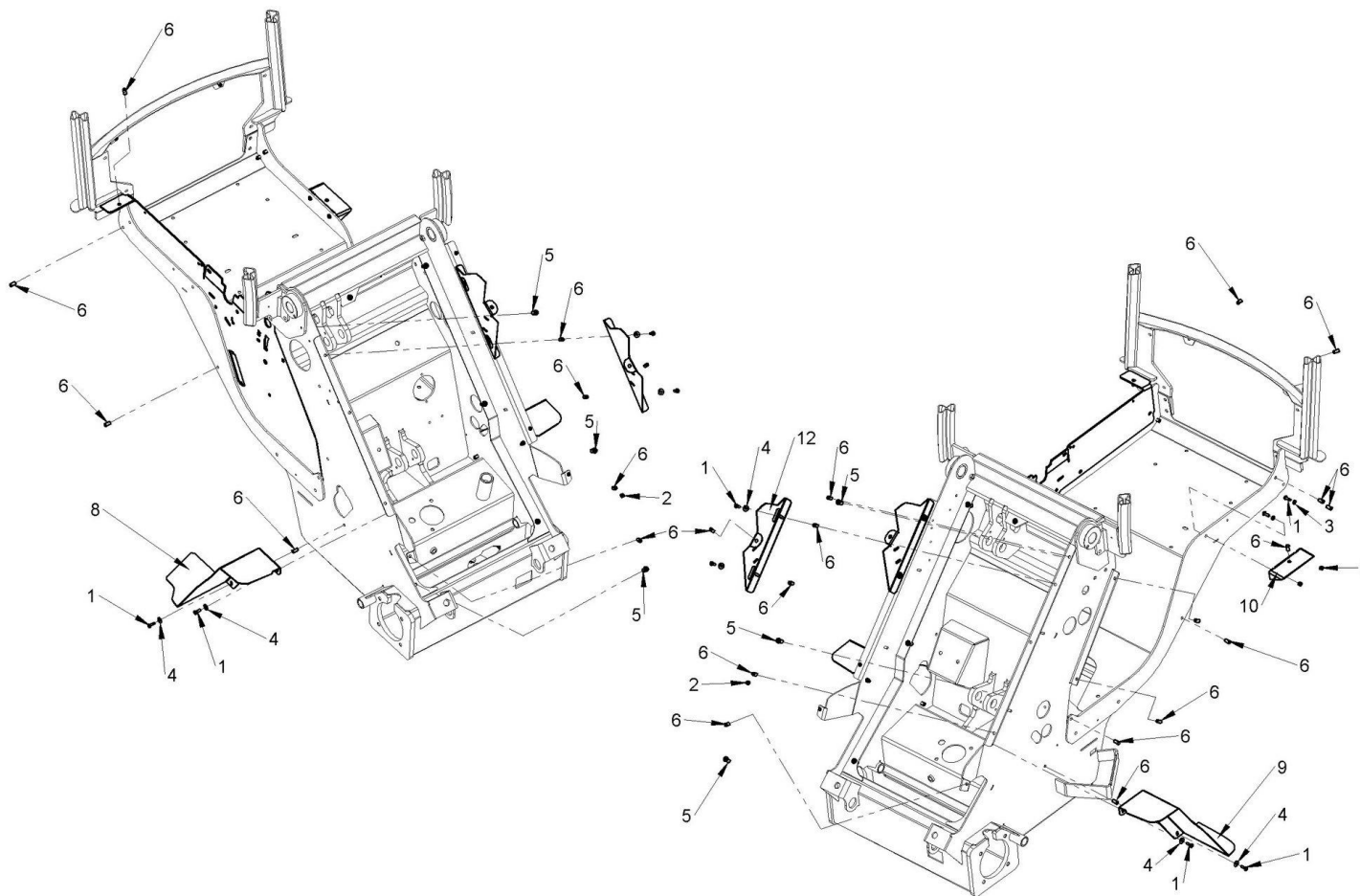
Component list [ TAV. 12 M1 5.3 FRONT COVER SUPPORT ]
