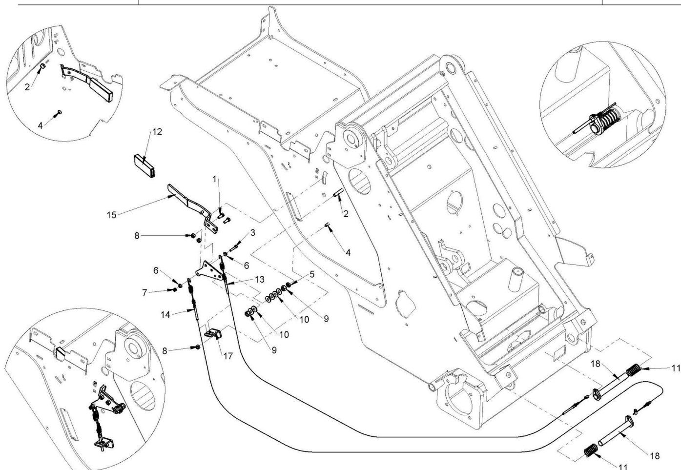
Component list [ TAV. 21 M1 5.3 HAND BRAKE ]
