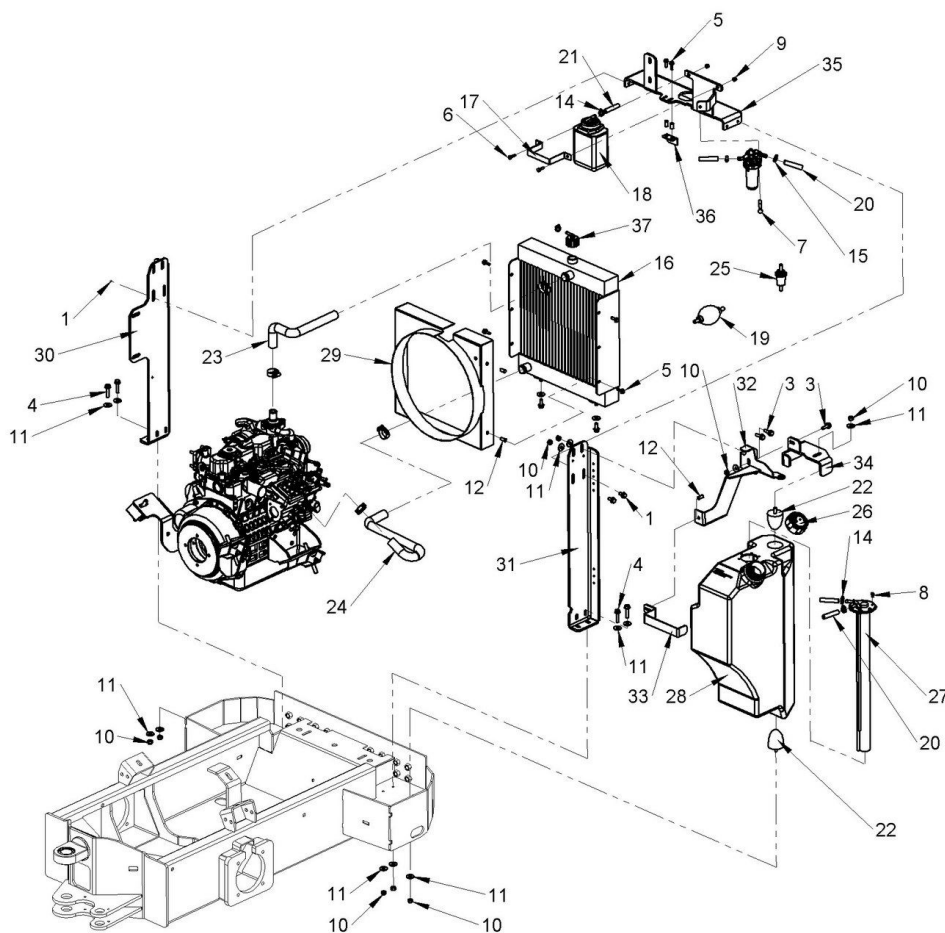
Component list [ TAV. 05 5.2 ENGINE COOLER AND FUEL TANK ]
