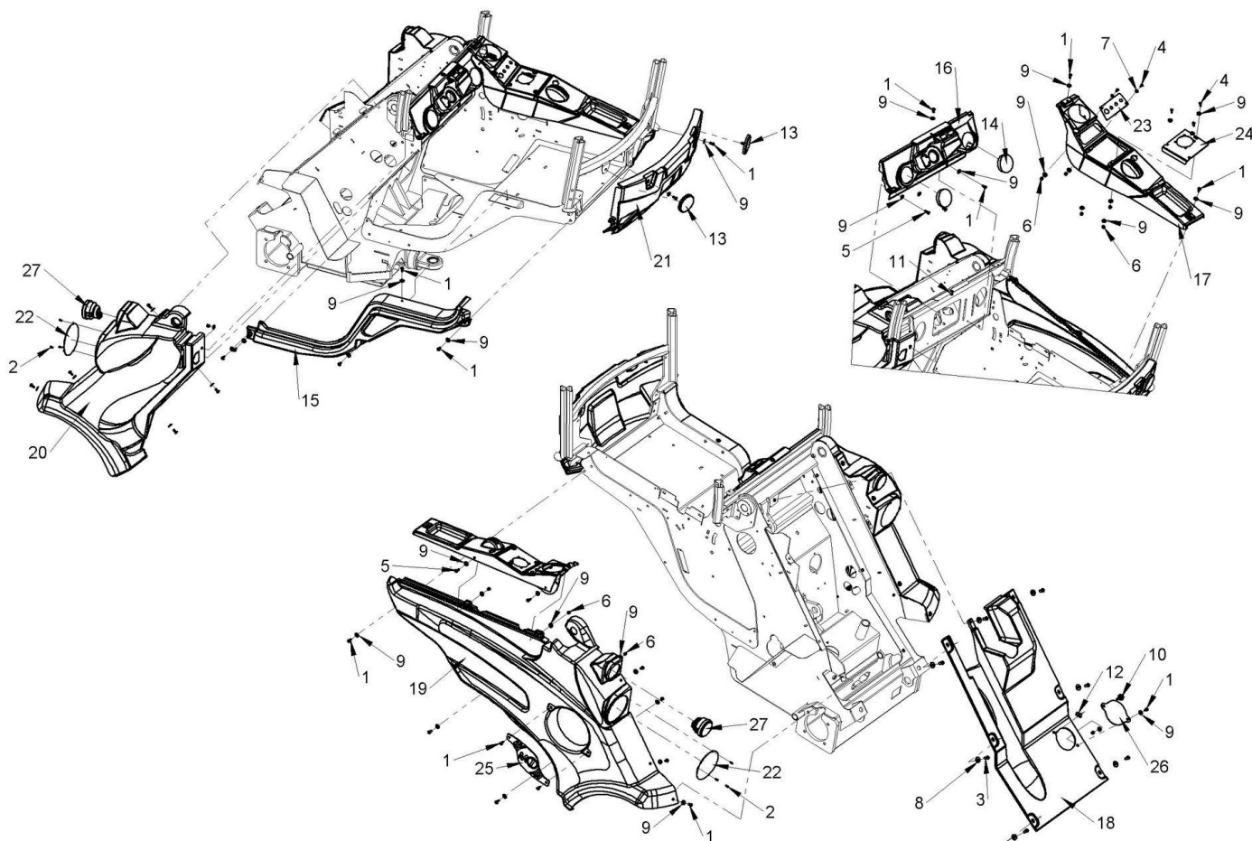
Component list [ TAV. 13 M1 5.3 FRONT PLASTIC COVER ]
