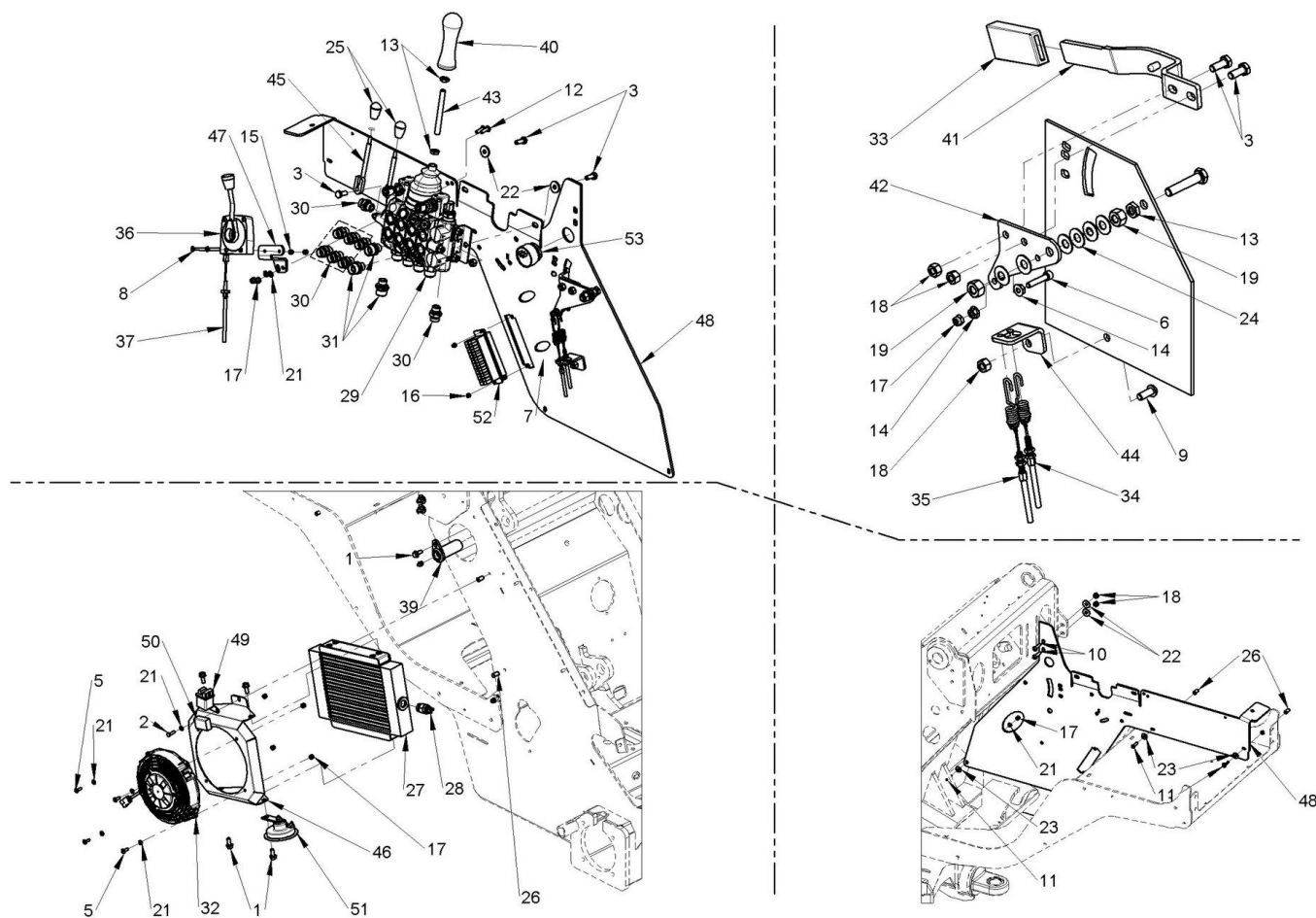
Component list [ TAV. 07 4.2 RIGHT SIDE ]
