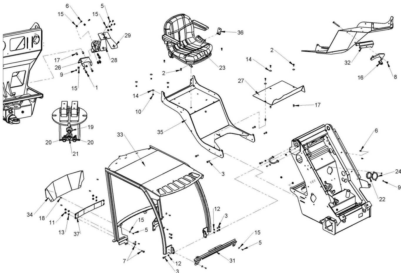
Component list [ TAV. 11 M1 5.3 SEAT ROLL-BAR AND PEDALS ]
